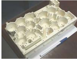
Plated Plastic RF Filter Housing
